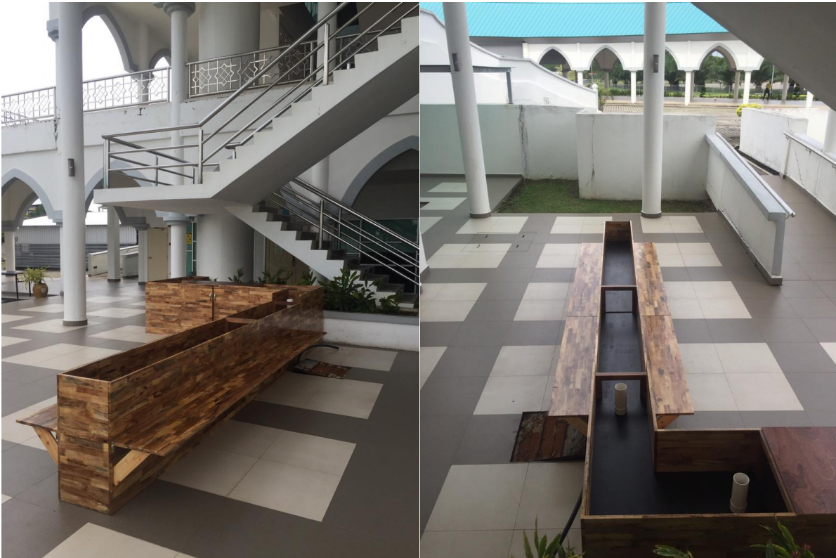
Figure 3: Aquaponic system
