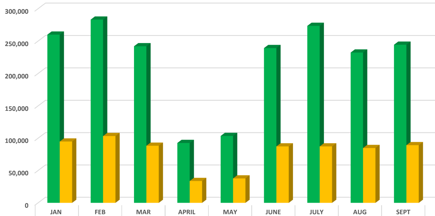
TOTAL ENERGY CONSUMPTION IN MAIN CAMPUS BY MONTH AT FPTV
